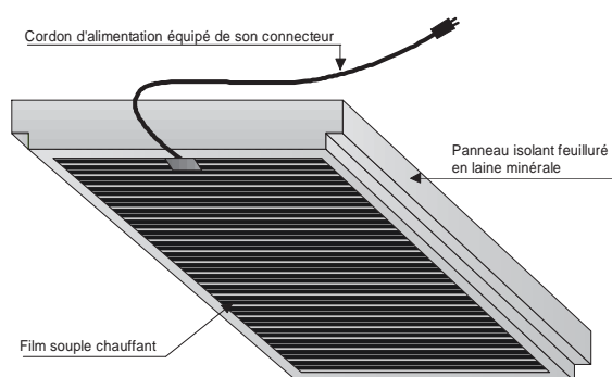
Figure 1 – Panneau chauffant
